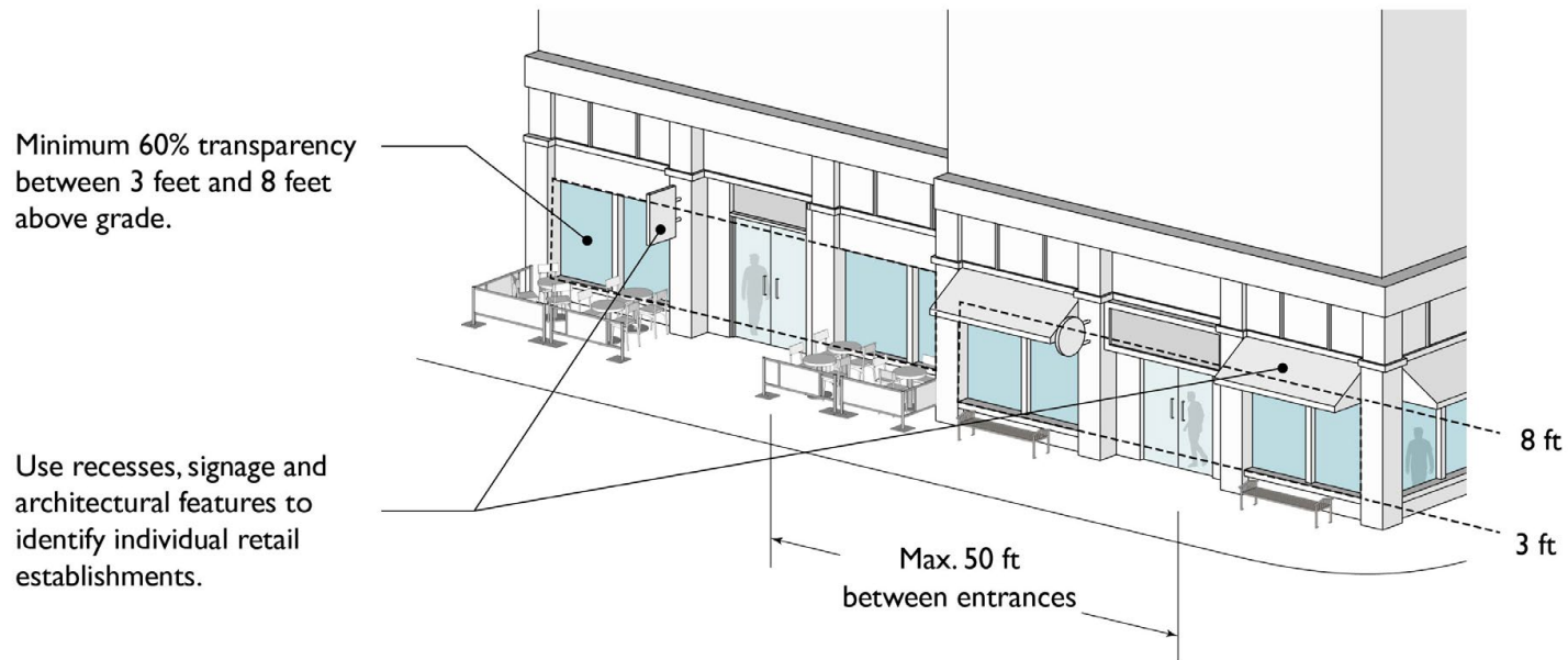
Figure 5-15: Ground Floor Retail Transparency
