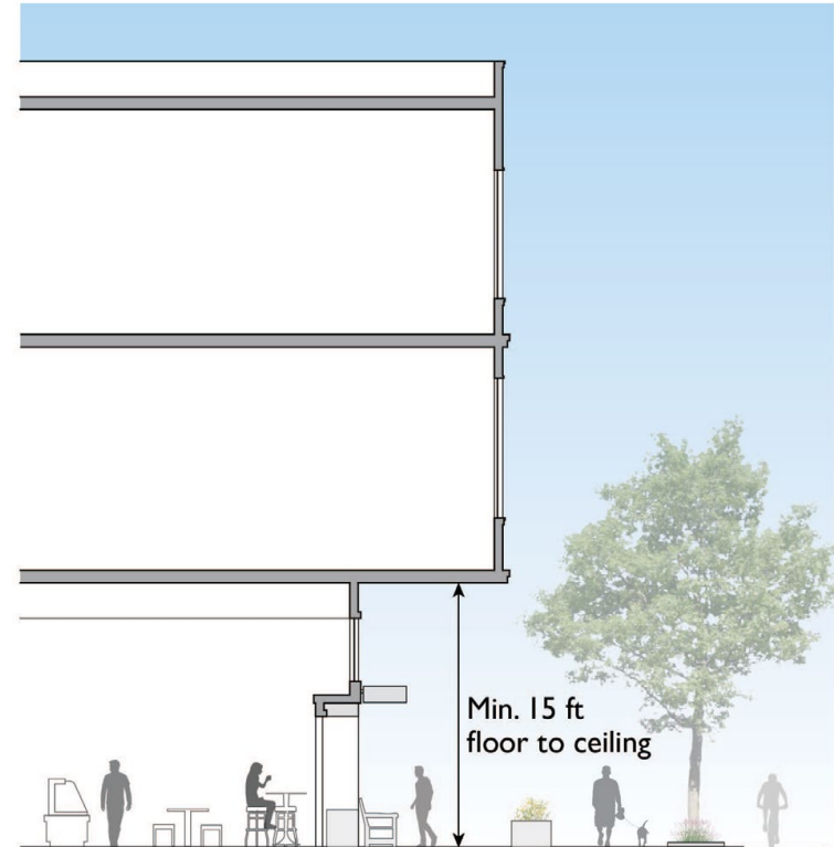
Figure 5-18: Ground Level Design - Ground Floor Commercial
