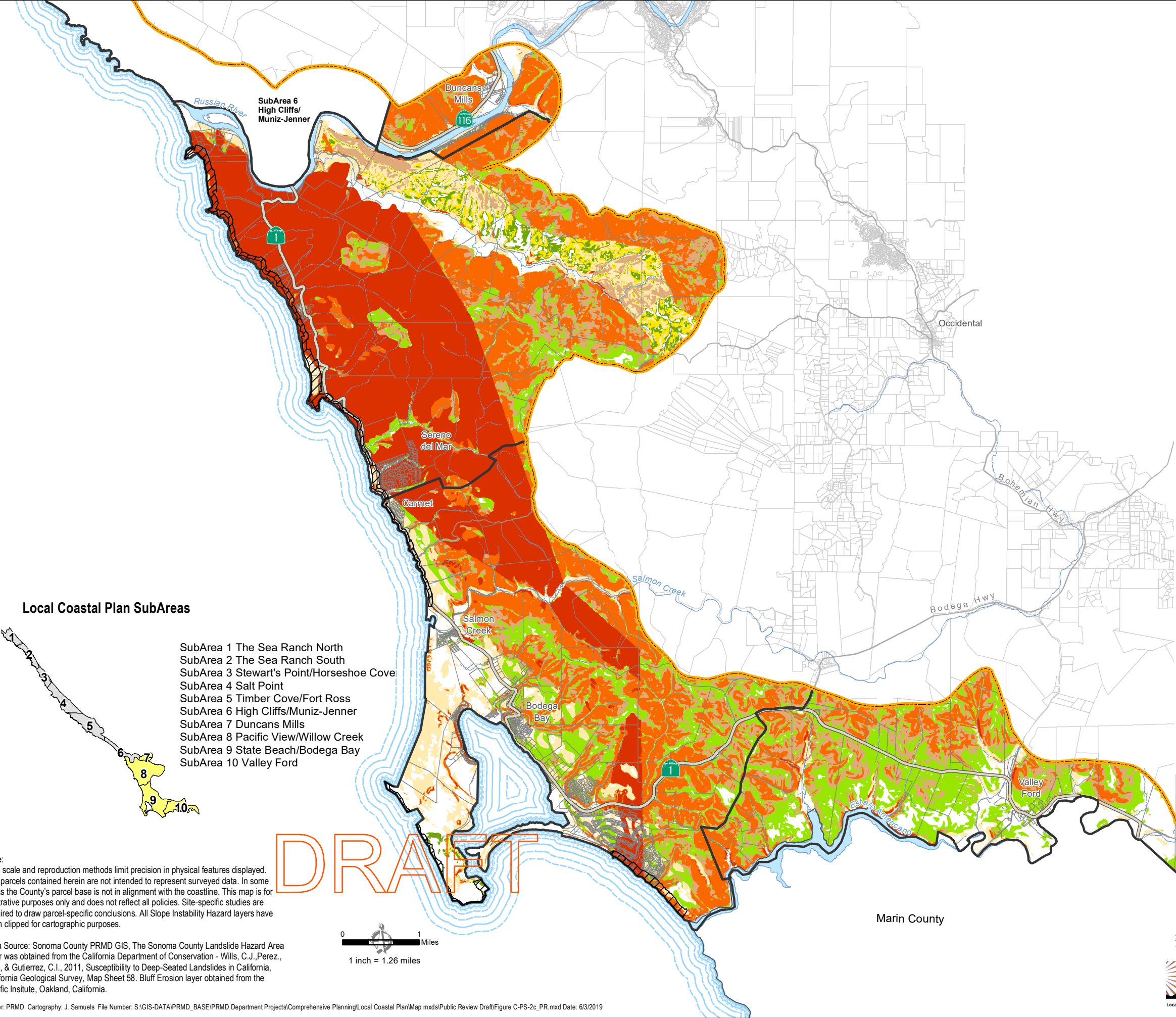
FIGURE C-PS-2c Slope Instability Hazards SubAreas 7 - 10
