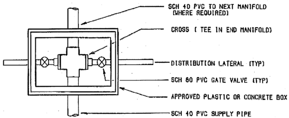
PLAN VIEW BALANCING VALVE DETAIL
