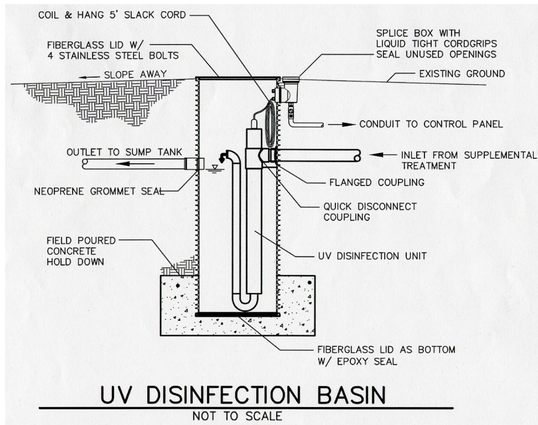
Figure 13.8g Disinfection Unit
