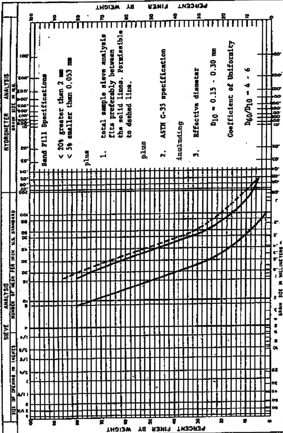
Figure 13.3d Mound Sand Criteria
